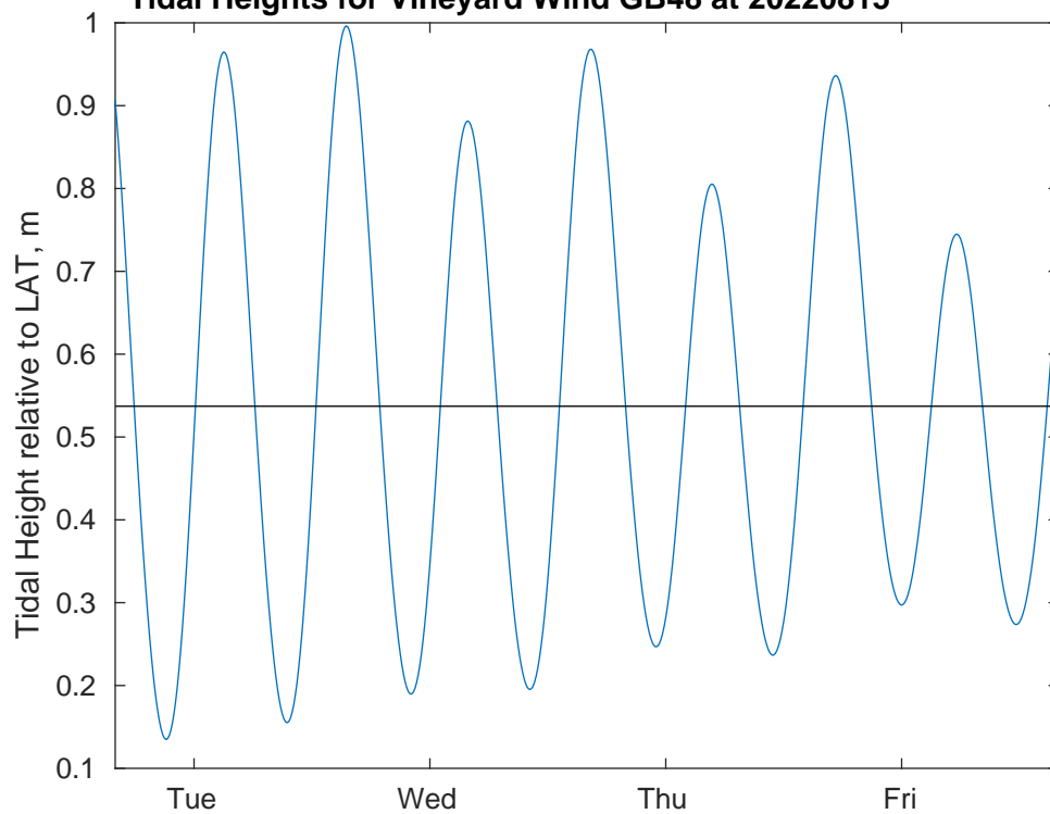
Tidal Heights for Vineyard Wind GB48 at 20220815
